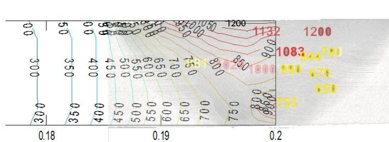
Fig. 4. Comparison between experimental and numerical maximum temperature measured and predicted at salient points within the weld region (experimental measurements - colour, numerical prediction - contour lines).
