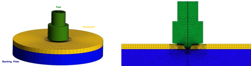
Fig. 6. (a) 3D mesh model; (b) cross section of the mesh centred on stirred zone and tool/workpiece interface.
