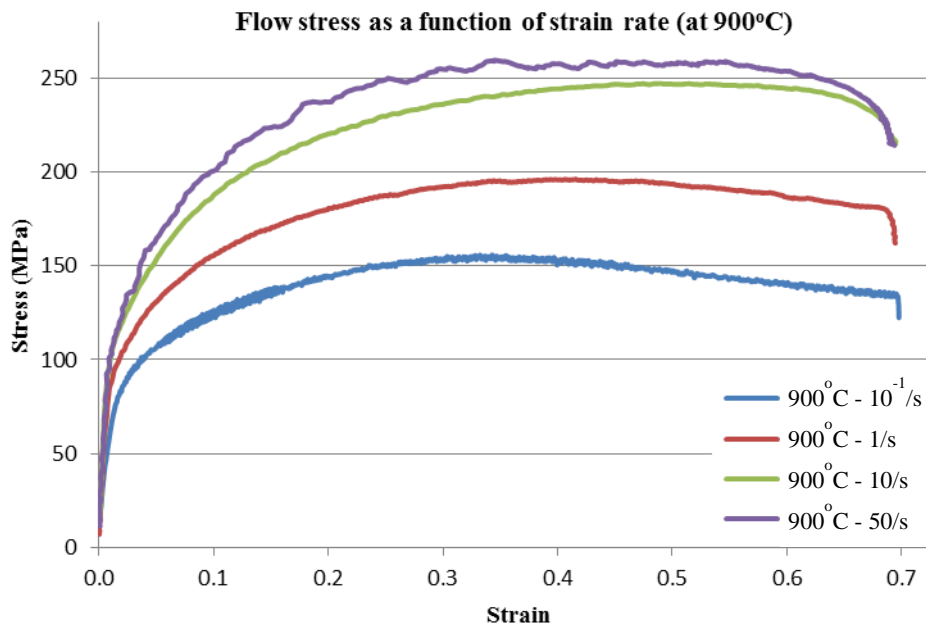
Fig. 3. Evolution of flow stress with increasing strain rate.
