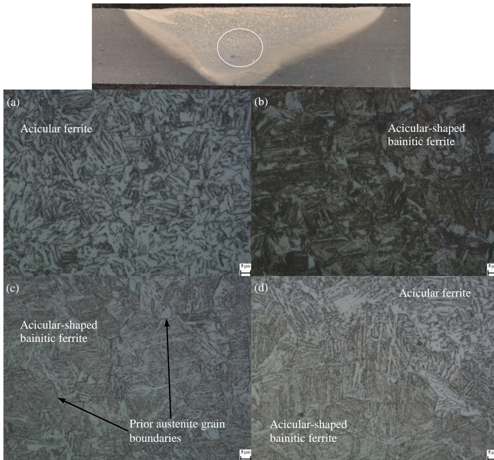
Fig. 2. Microstructure of mid-TMAZ [x1000, Etched] (a) Slow; (b) Intermediate 1; (c) Intermediate 2; (d) Fast
