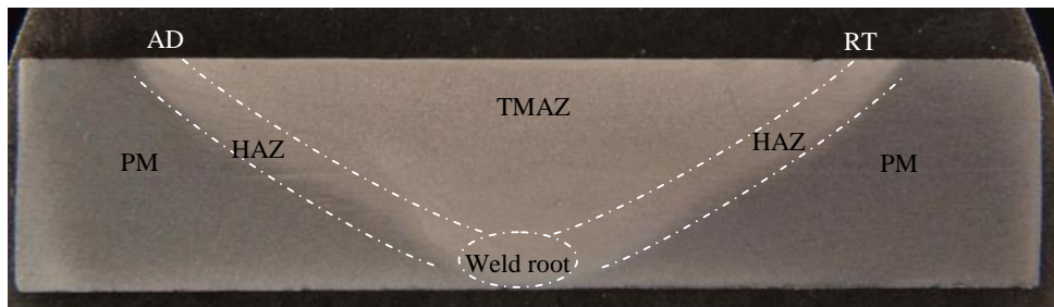
Fig. 1. A typical macrograph of the friction stir weld region
