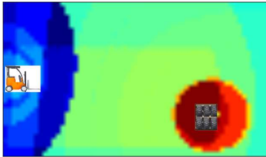
Fig. 5: Heat map showing the learned distribution for “to the tire pallet.” probability.
