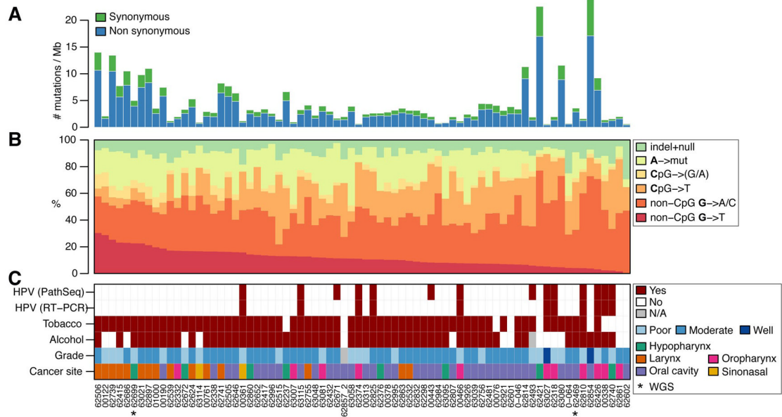
Fig. 1. Mutation rates, base substitution frequencies, and rearrangements in head and neck cancers. (A) Rate of synonymous and non-synonymous mutations, expressed in mutations per megabase of covered target sequence. Non-synonymous mutation rates range from 0.43 to 17.1 mutations/megabase (mean = 3.3). (B) Breakdown of individual base substitution rates used for mutation significance, for the same samples as panel (A). The samples were ordered by the rate of G→T transversions, which are indicative of smoking-induced mutations. (C) Key clinical parameters for the samples described in panels (A) and (B) (table S10). The first row indicates HPV detection by sequencing, the second row indicates HPV detection by real-time PCR.
