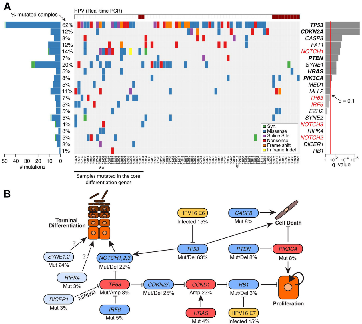
Fig. 3. Genetic disruption of a squamous differentiation program in head and neck cancers. (A) Heatmap representation of individual mutations present in a series of 74 tumors, represented in columns. (Top) HPV status by tumor. (Middle) Matrix of mutations in individual genes by type of mutation and tumor. (Left) Number of mutations in each gene. Percentages represent the fraction of tumors harboring at least one mutation in the specified gene. (Right) Deleted recurrently mutated genes ranked by q-value. Genes that define the core differentiation cluster are listed in red. (B) Proposed partial wiring diagram of the molecular circuitry of HNSCC. Blue, loss of function; red, gain of function. Numbers listed beneath each protein represent the fraction of tumors harboring mutations, amplifications, or deletions in the corresponding genes.
