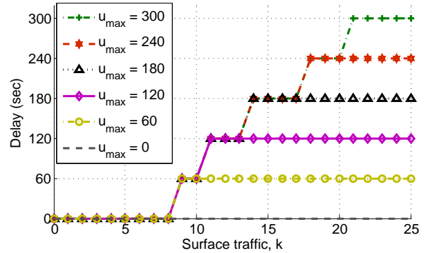
Fig. 7. Optimal policies for Boston Logan, when departures take place from Runway 27.
