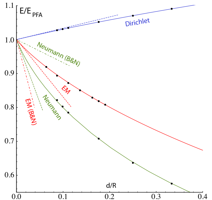
FIG. 1: Casimir energy normalized to PFA energy as a function of d/R for the sphere-plate configuration: Numerical data (dots, from Ref. [10]), Padé approximants (solid curves) and the first correction to the PFA (dashed lines). Also shown are the linear slopes (dashed-dotted lines) computed by BN [11, 12].
