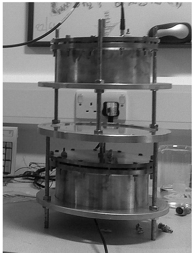
Figure 2: The copper pillbox cavities on their test stand.
