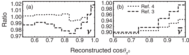
FIG. 11. (a) The ratio of the \nu_\mu NC 1\pi^0 angular cross section extracted using the coherent production models in [4] (dotted line) and [3] (dashed line) compared to the principal result extracted using the R-S model. (b) The same for the \bar{\nu}_\mu NC 1\pi^0 cross section.
