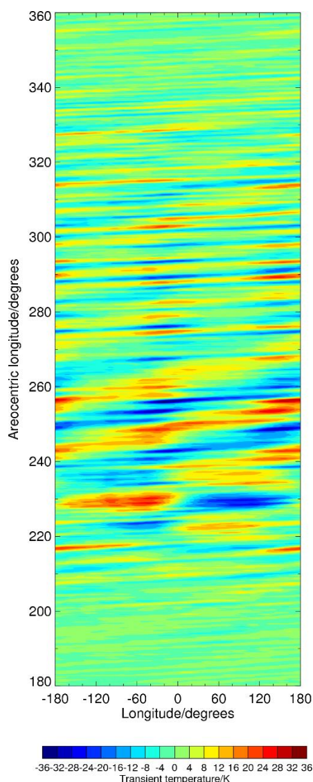
Figure 1: Transient temperature on the 50 Pa pressure surface ( \sim 25 km altitude) at 62.5^\circ\text{N} over the period, L_S=180^\circ – 360^\circ (northern autumnal to vernal equinox), of MY 24.
