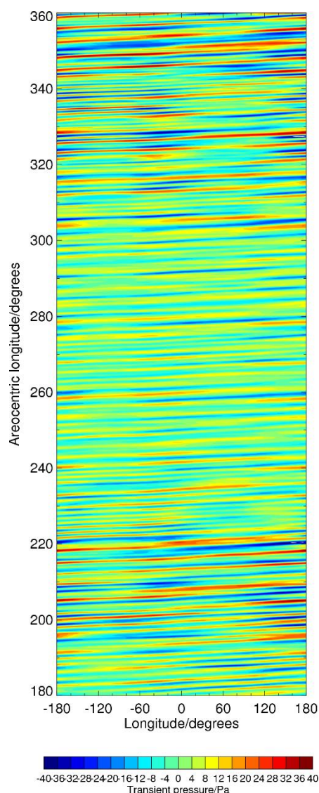
Figure 2: Transient mean zero datum-level pressure, over the same latitude and time range as Fig. 1.
