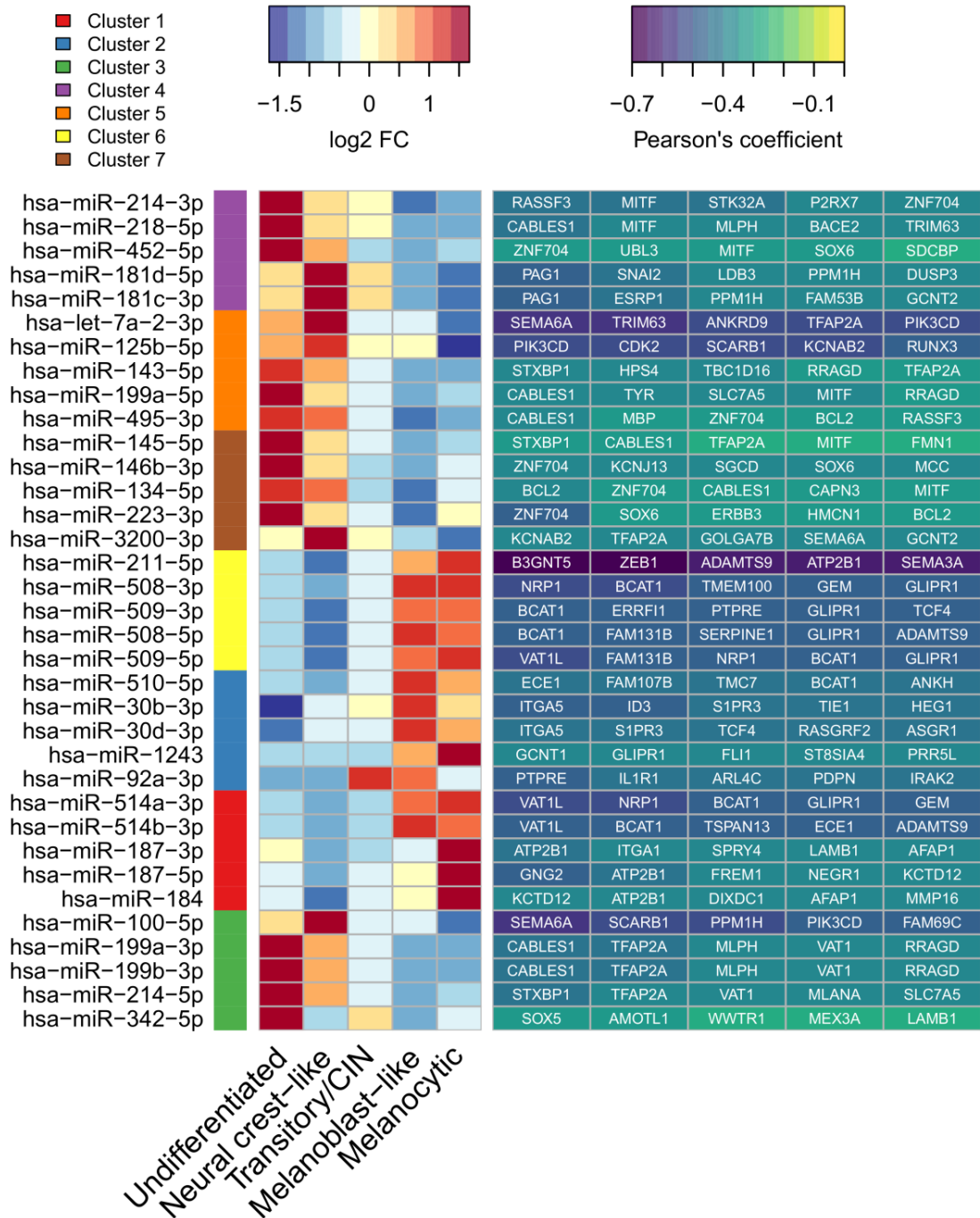
Figure 4.28. Top-differentially expressed miRNAs and related targets. The heatmap on the left shows the log 2 fold changes across consensus subtypes of the top-5 most significantly differentially expressed miRNAs for each cluster identified in Figure 15A. The heatmap on the right report the top-5 anti-correlated predicted target genes of the miRNAs on the left. The color scale is proportional to the Pearson's correlation coefficient of the miRNA-target pair.
