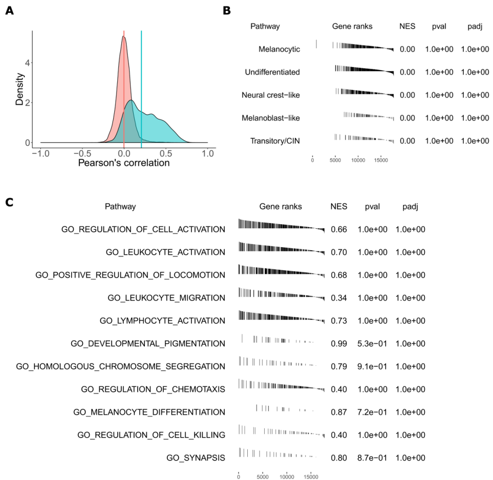
Figure 4.23. Integrative analysis of RNA-Seq and copy number data. A) Distribution of the Pearson's correlation values the expression of each gene and its copy number log 2 ratio. The green curve is the observed distribution, compared to a random distribution obtained by randomly shuffling the genes 1000 times. B-C) Enrichment plots for selected gene sets tested against the list of genes pre-ranked according to the Pearson's correlation coefficient. The "Gene ranks" column shows the location of the genes included in each pathway along the pre-ranked gene list. NES: normalized enrichment score; padj: adjusted p-value.
