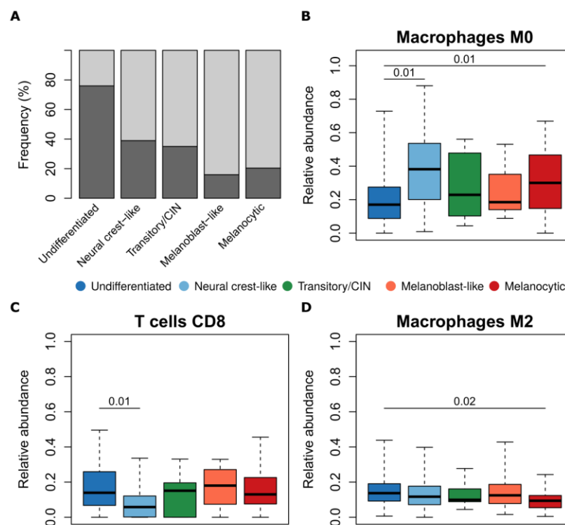
Figure 4.12. Association between immune infiltration status defined by CIBERSORT and consensus subtypes. The percentage of immune samples (CIBERSORT p-value < 0.05 , dark grey) and non-immune samples (CIBERSORT p-value \geq 0.05 , light grey) are presented for each subtype. B-D) Box plots of CIBERSORT-inferred cell proportions for the cell subpopulations with an ANOVA p-value < 0.05 . Reported p-values for pair-wise comparisons were calculated using Tukey’s post-hoc test.
