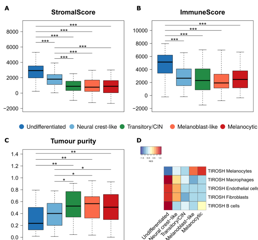
Figure 4.11. Microenvironment contribution to the gene expression of consensus subtypes. A-B) Box plot of the stromal and immune score calculated from the expression of specific markers using the ESTIMATE package. C) Tumour purity inferred from the combination of the stromal and immune score. P-values were obtained with ANOVA followed by Tukey’s post hoc test. ***: p < 0.001 ; **: p < 0.01 ; *: p < 0.05 . D) Heatmap of the average NES calculated using GSVA for cell-specific markers in each subtype.
