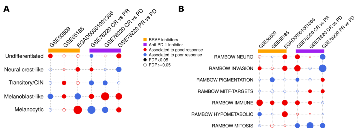
Figure 4.18. Assessment of the predictive value of melanoma transcriptional state signatures in clinical tumours. A-B) Bubble plots showing the association of selected signatures and response to anti-MAPK and anti-PD-1 therapy in publicly available datasets. The size of each circle is proportional to the normalized enrichment score calculated by GSEA.
