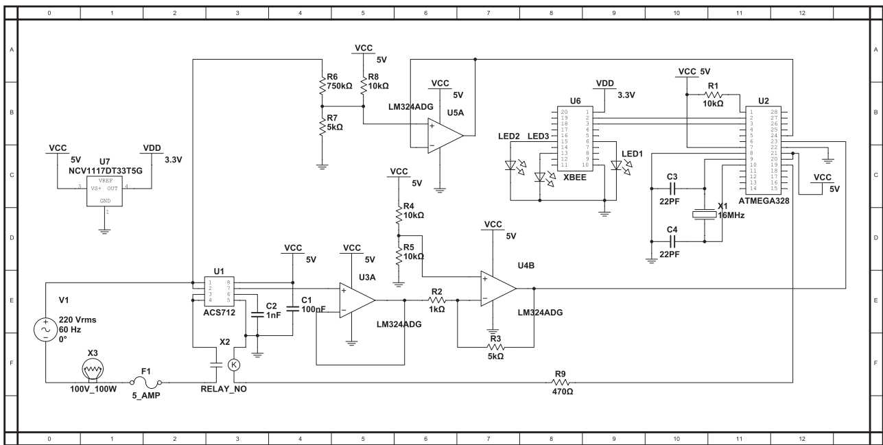
Fig. 3. Slave circuit hardware.
