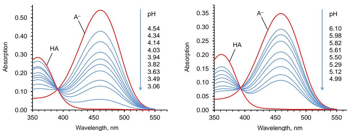
Fig. 3 Absorption spectra of 2,6-dinitro-4- n -dodecylphenol in 0.01 M TX 100 solution, 0.1 M NaCl (a) and 0.01 M SDS solution, 0.1 M NaCl (b).
