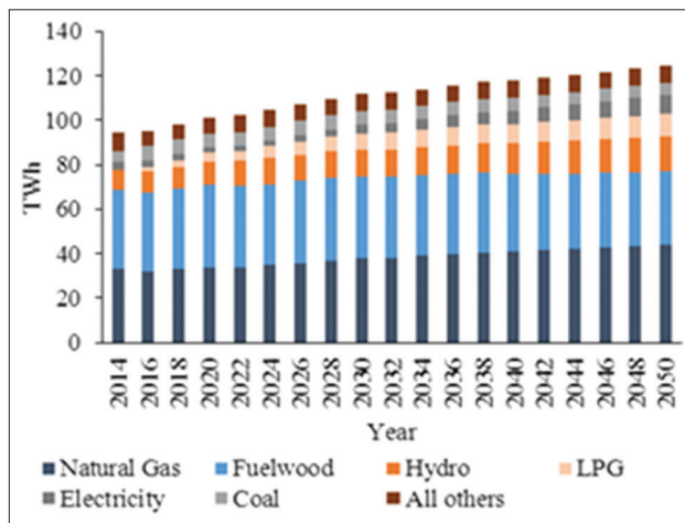
Figure 7: Primary energy consumption prospective. Residential sector. Baseline scenario
