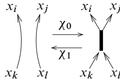
Figure 5: Maps \chi_0 and \chi_1
