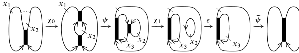
Figure 16: Homomorphism \Phi . To avoid cluttering only some marks are shown
