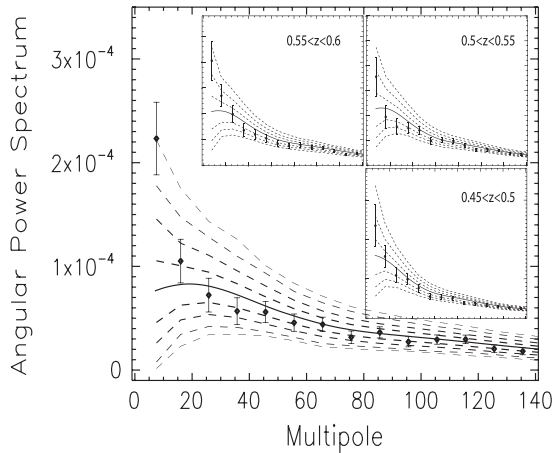
FIG. 1. The angular power spectra C_\ell measured in the SDSS photometric MegaZ DR7 luminous red galaxy survey. The panels relate to four redshift bins with width \Delta z = 0.05 from z = 0.45 to z = 0.65 . The best fit theoretical spectra (solid lines) are excellent matches to the data including multipoles up to \ell \sim 500 . However, the largest angular scales are observed to be anomalous; the dashed lines correspond to 1 \rightarrow 4\sigma derived from simulations. This is particularly severe in the highest redshift bin (main panel), which is \sim 4\sigma .
