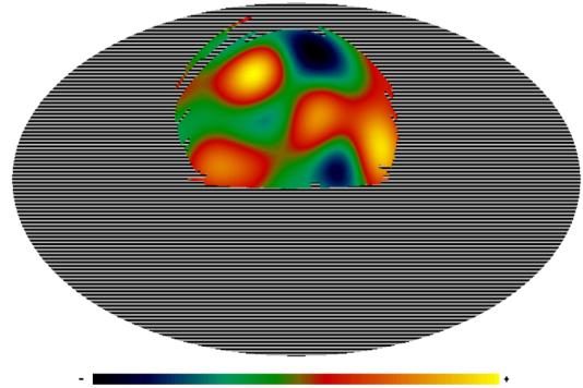
FIG. 2 (color online). A visualization of the measured underlying field within the surveyed region on the sky. Only contributions from \ell = 4 \rightarrow 10 in the most anomalous multipole and redshift band are included.
