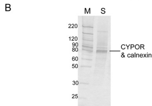
Figure S1 Purification of NADPH-dependent NO consumption
