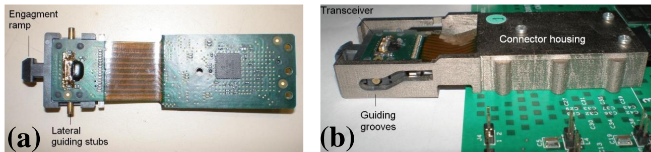
Figure 7: (a) Parallel optical transceiver circuit with lateral guiding stubs. (b) Connector housing with transceiver circuit incorporated
