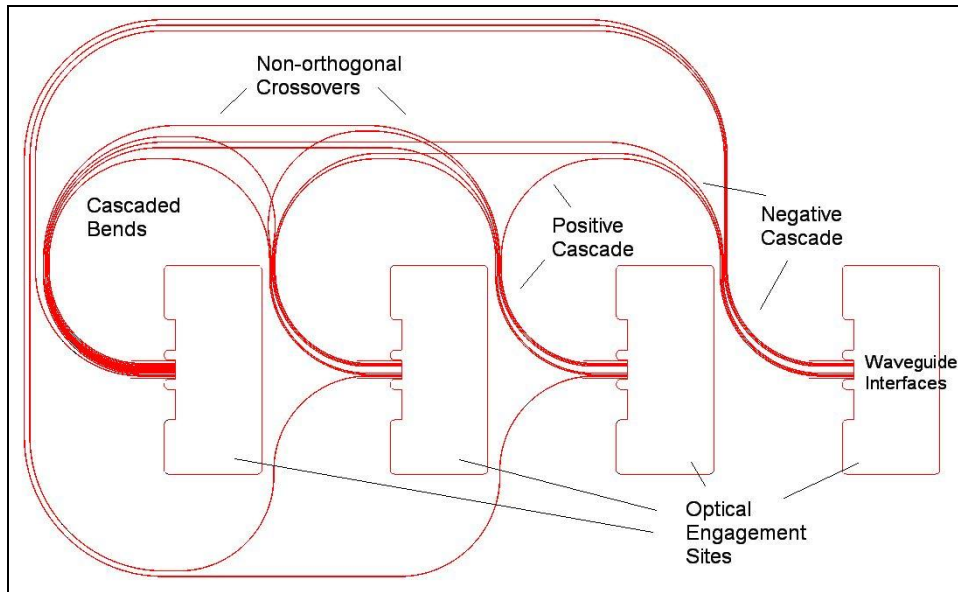
Figure 3: Optical waveguide layout including cascaded bends and non-orthogonal crossovers
