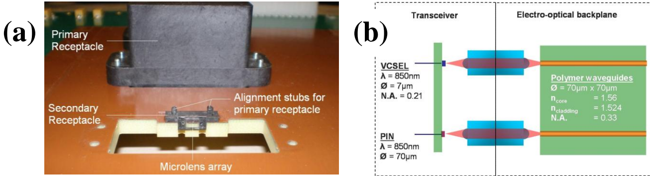
Figure 8: (a) Primary and secondary receptacles assembled onto electro-optical backplane. (b) Dual lens coupling interface between transceiver and electro-optical backplane
