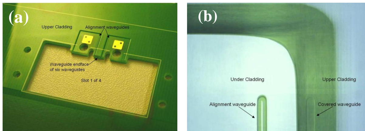
Figure 4: (a) Clearance areas in upper cladding layer to provide mechanical access for optical connector receptacle and waveguide end facet
