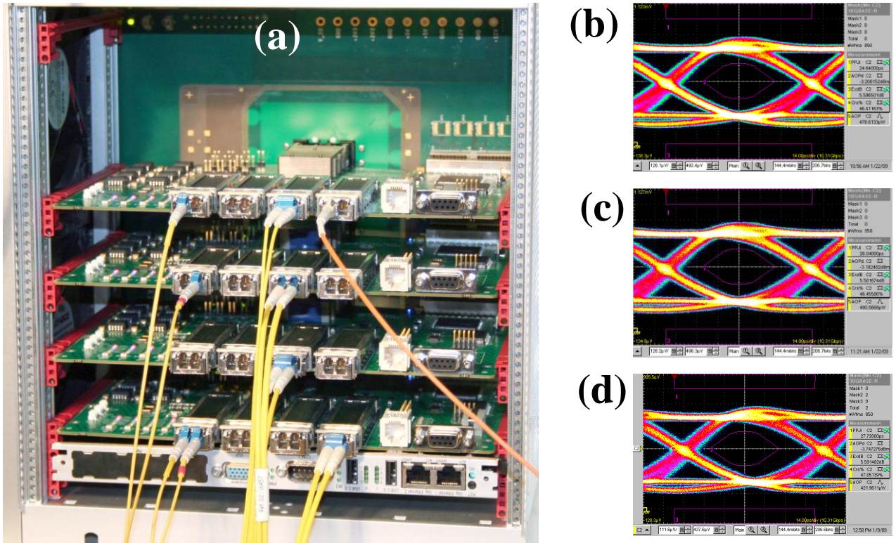
Figure 10: (a) Demonstration platform comprising a Compact-PCI chassis with single board computer and a hybrid electro-optical backplane.
