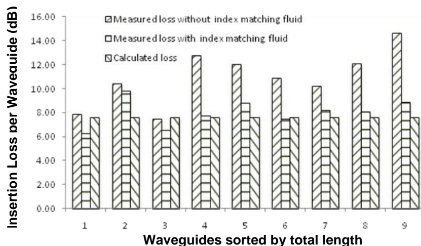
Figure 5: Projected and measured values for insertion loss on a group of 9 waveguides
