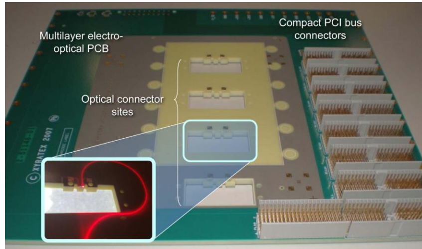
Figure 2: An electro-optical backplane and a waveguide illuminated with 635 nm light exiting one of the connector slots
