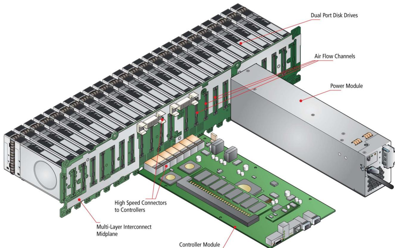
Figure 1: Modern data storage array with hard disk drives connected to one side of the backplane (or midplane) and controller boards and power supplies connected to the other
