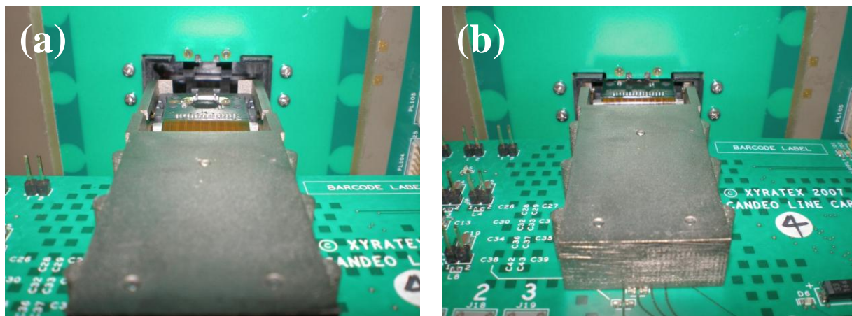
Figure 9: (a) First stage of optical backplane connection process: connector housing is slotted into larger backplane receptacle and coarsely aligned with backplane lens array. (b) Second stage: optical platform lens array is butt-coupled to backplane lens array.
