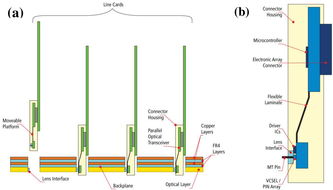
Figure 6: (a) Optical backplane connection scheme; active pluggable connectors housed on the edge of peripheral line cards engage with the embedded optical layer in the backplane PCB. (b) Active optical connector comprising a parallel optical transceiver, connector housing and engagement mechanism.
