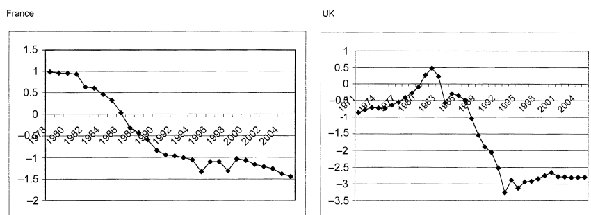
FIGURE 2. Results from first-stage regressions for UK and France.
