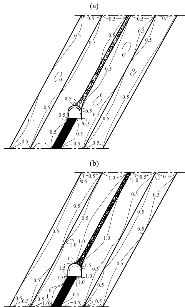
Figure 11. Static field of tangential stresses in the vicinity of the haulage gate in the method of the mining pressure controlling in face with goaf stowing: (a) with the filling mass hardness C = 35 \text{ N/m} ; (b) the same, C = 84 \text{ N/m}
