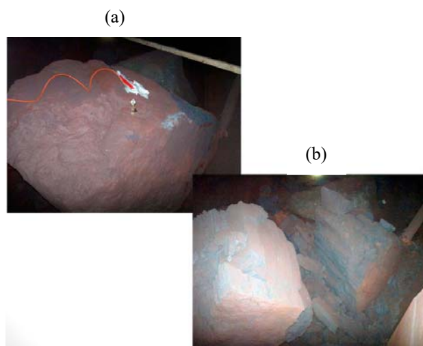
Figure 2. Explosion results with the use of a pressure charge of Ukrainit-P EE of P – S type while breaking oversize material: (a) is a pressure charge on oversize material ((a) watch is used for scale); (b) is the explosion result (general view)
