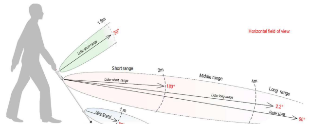
Fig. 6. Coverage of the different range sensors integrated in the white cane
