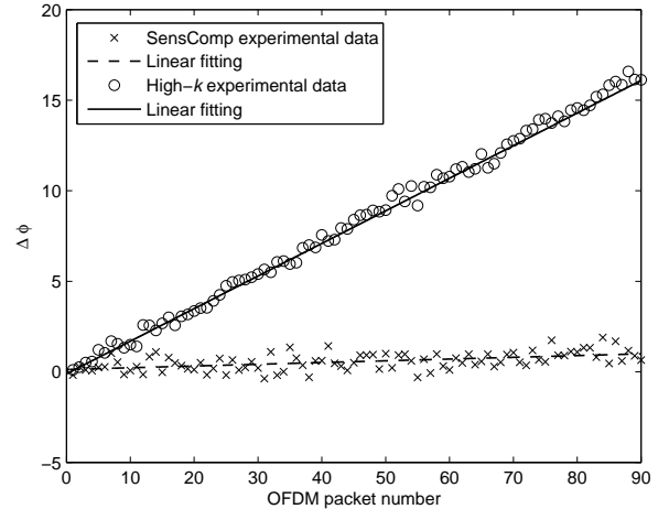
Fig. 13. The trend of the group phase offset when using SensComp and high- k ultrasonic transducers with their individual linear fittings.
