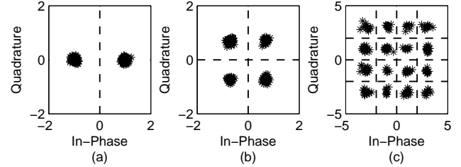
Fig. 2. Simulated OFDM signal constellation diagrams for an SNR of 5 dB. (a) BPSK, (b) QPSK, and (c) 16-QAM. The detection boundaries are indicated by dashed lines.
