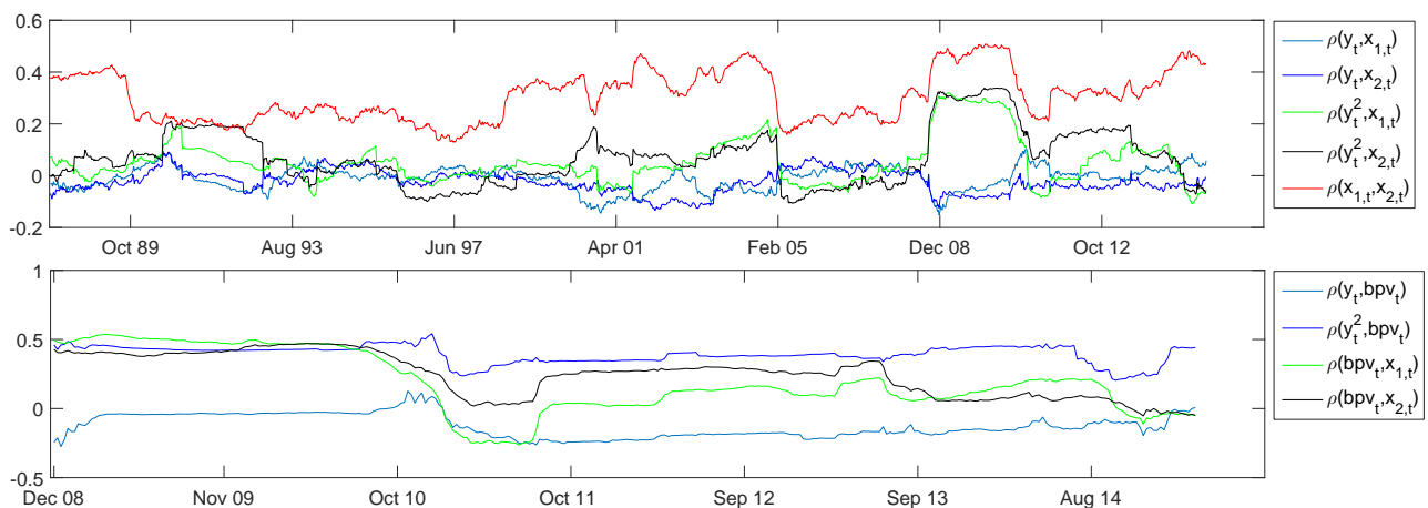
Figure 1: The dynamic correlations, \rho(\cdot) , of the variables y_t , y_t^2 , bpv_t , x_{1,t} , x_{2,t} . The linear correlation coefficients were computed using a rolling window procedure with a window size of 500 observations and a step of 5 days.
