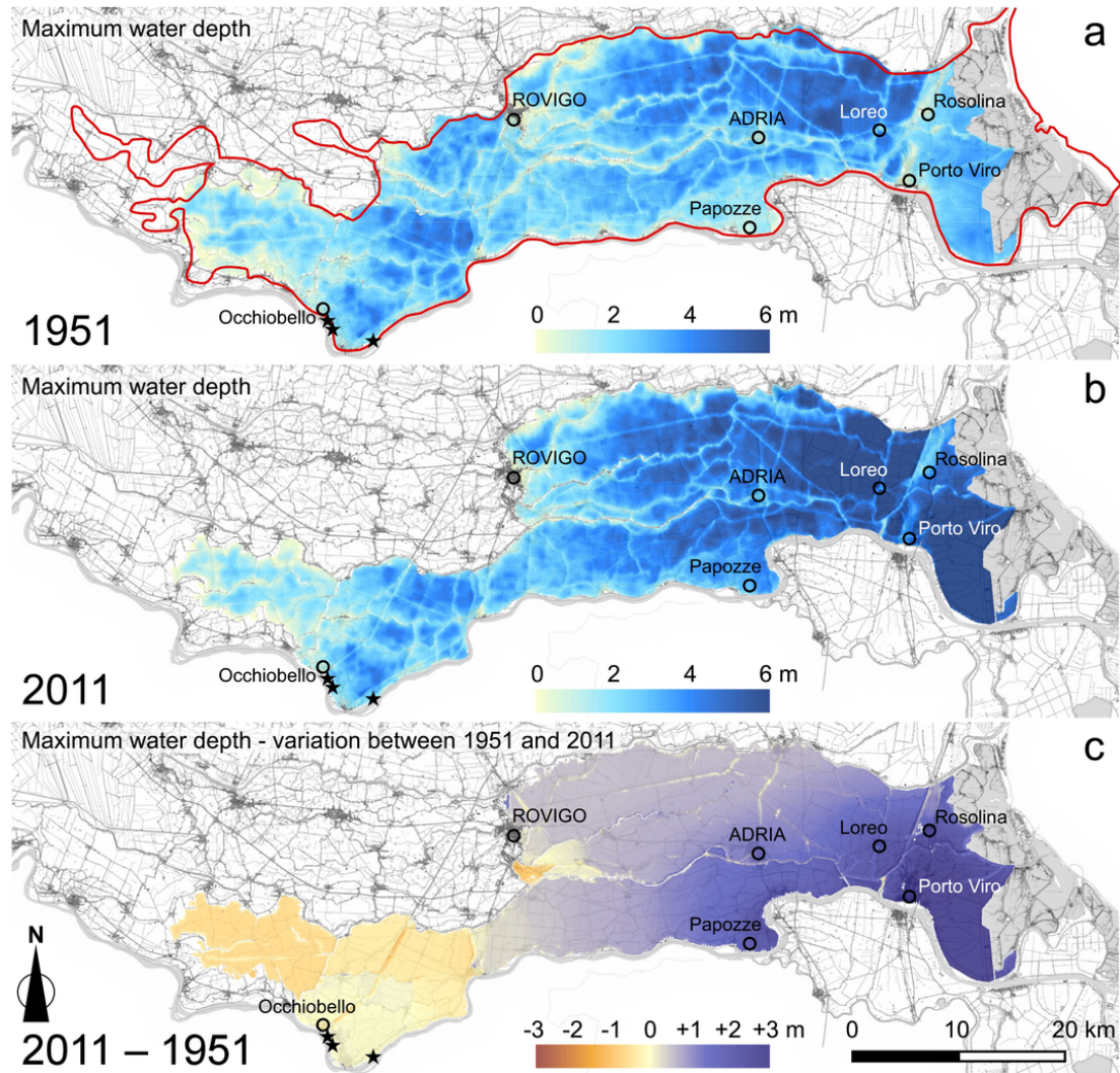
Fig. 7. Maximum water depth for the 1951 (a) and the 2011 (b) scenarios, and difference between the two (c). The red line in panel a bounds the surveyed flooded area in 1951; black stars denote the position of the three levee breaches. (For interpretation of the references to color in this figure legend, the reader is referred to the web version of this article.)
