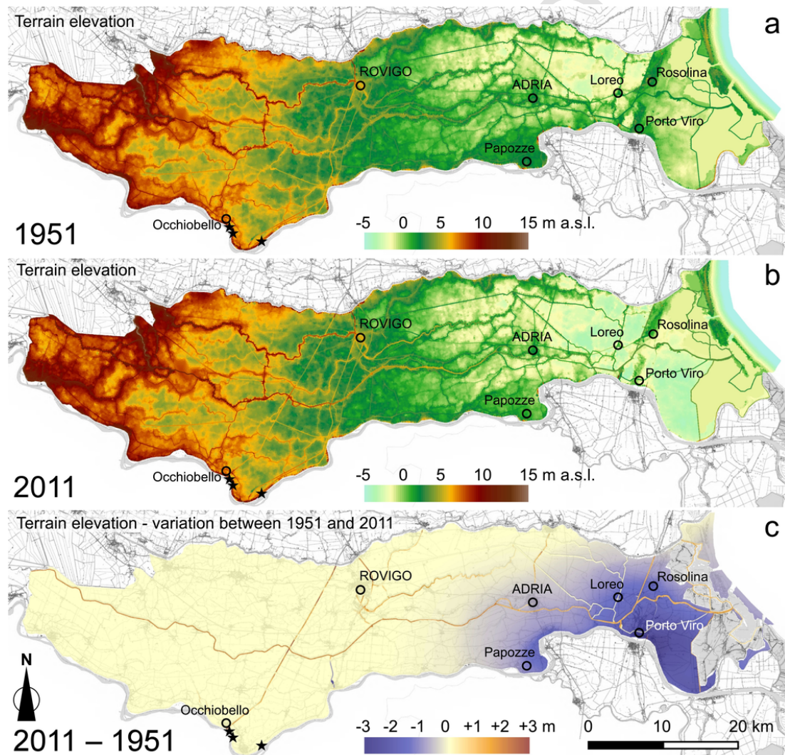
Fig. 5. Terrain elevation (m.a.s.l.) concerning 1951 (a) and 2011 (b), and variation in terrain elevation between the two time frames (c); black stars locate the three levee breaches. (For interpretation of the references to color in this figure, the reader is referred to the web version of this article.)
