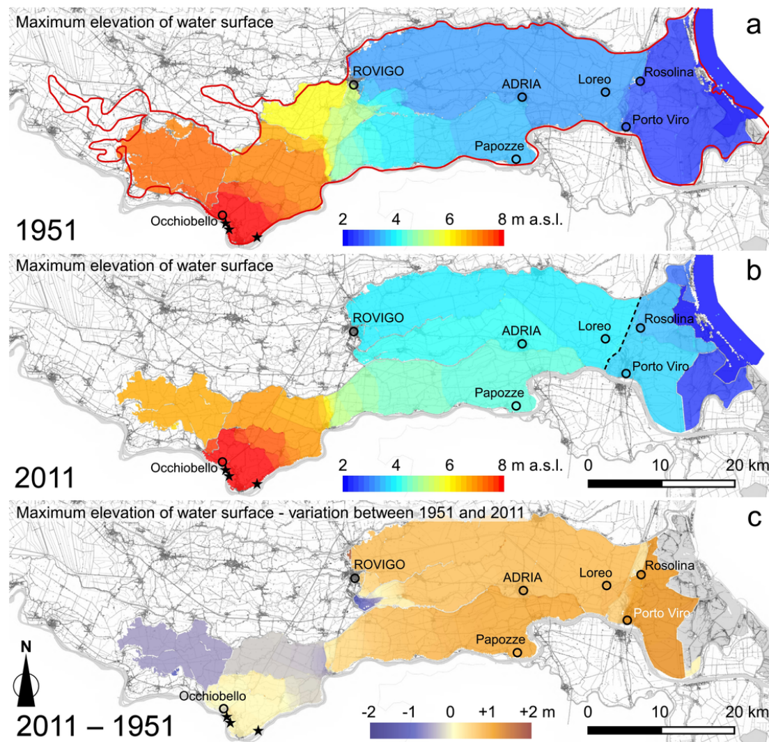
Fig. 6. Maximum elevation of the water surface for the 1951 (a) and the 2011 (b) scenarios, and difference between the two (c). The red line in panel a bounds the surveyed flooded area in 1951; the dashed line in panel b denotes the Po-Brondolo canal; black stars denote the position of the three levee breaches. (For interpretation of the references to color in this figure legend, the reader is referred to the web version of this article.)
