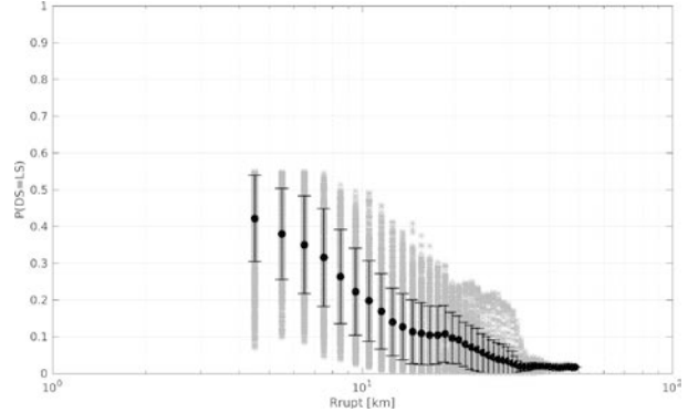
Figure 8. Normalized probability of damage state (DS) being equal to Life Security (LS) versus the closest distance to the fault rupture (Rrupt). Grey stars denote the P(DS=LS) for each monitored points within the Beijing area, while filled black dots represent the mean of P(DS=LS) at a given distance and the black bars represent the corresponding standard deviation.
