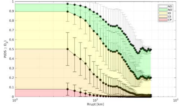
Figure 9. Normalized probability for all damage states (DS) versus the closest distance to the fault rupture (Rrupt). The different colors denote the P(DS=D_s) for each VRG point (white: no damages – ND; green: very light damages, normal operation – NO; yellow: light damages, immediate operation – IO; orange: moderate damages, life security – LS; red: severe damages, collapse prevention – CP), while filled black dots represent the mean of P(DS=D_s) at a given distance and the black bars represent the corresponding standard deviation.
