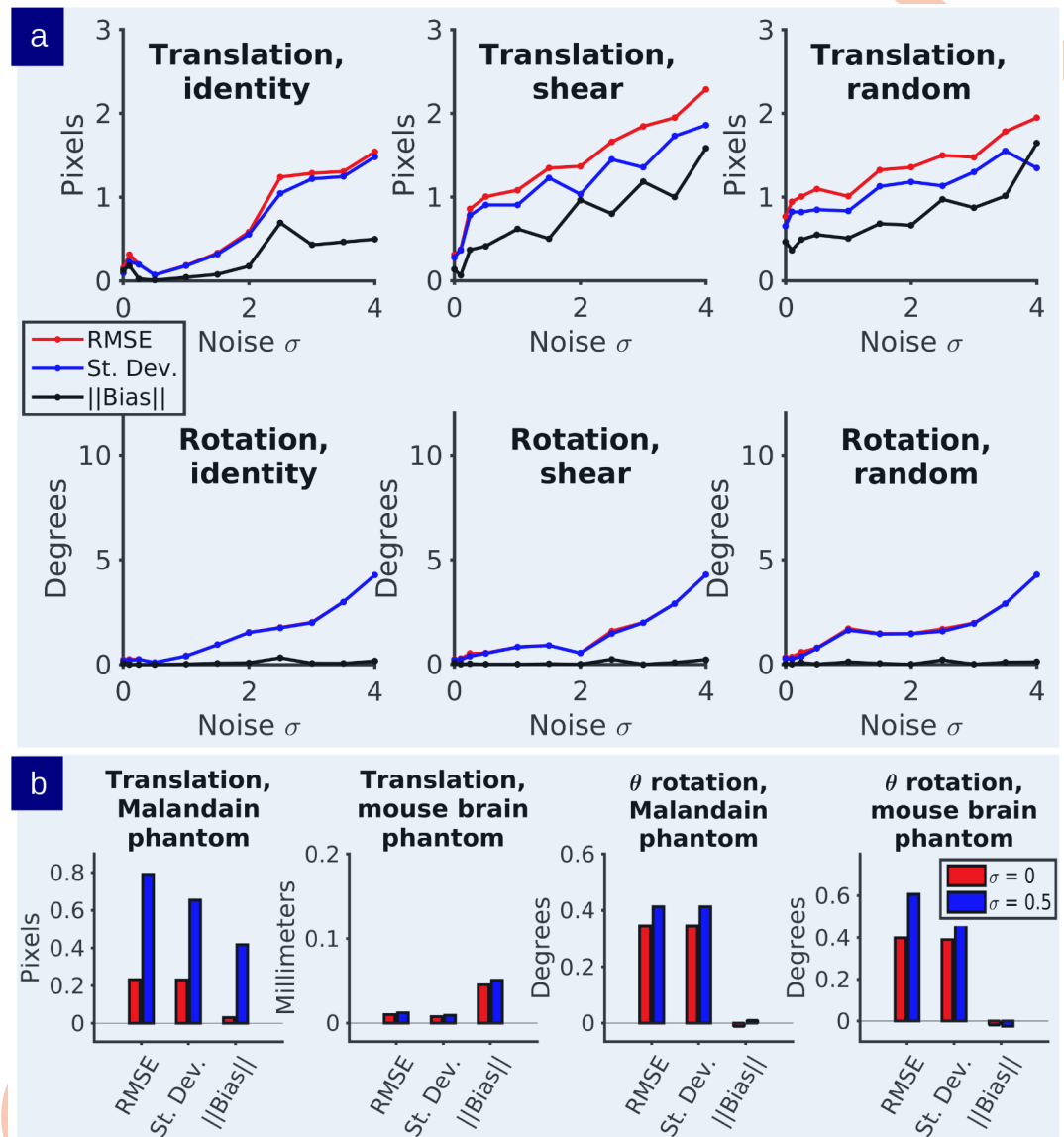
Fig 7. Evaluation of estimator MSE, variance, and bias. a) Statistics on the translation-rotation estimators for noise levels varying initial conditions. b) Statistics on the rigid motion estimators where the section jitter was added in a random fashion.
