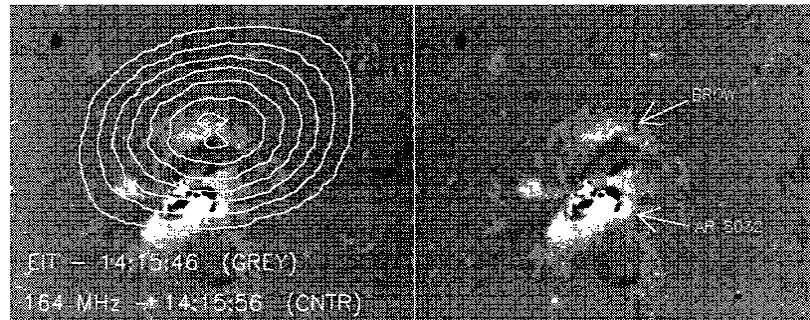
Figure 3.3: Superposition of 164 MHz type II burst contours on an EIT difference image. The EIT “brow” (S-wave) can be clearly seen to the north of AR 8032. Figure from Gopalswamy et al. (2000). Permission to reproduce this figure has been granted by the Astronomical Society of the Pacific.
