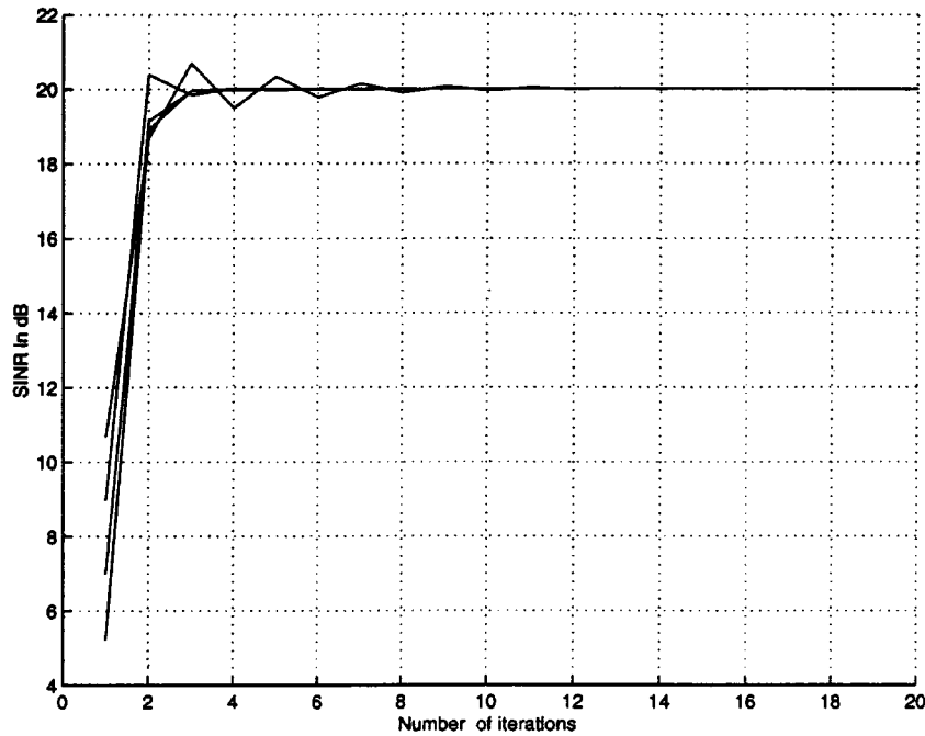
Fig. 10. Convergence of SINR for all the links for Example 1 (4 + 4 SBM/OFDM, Q = 4 and \Gamma_0 = 20 dB).
