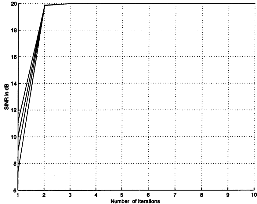
Fig. 11. Convergence of SINR for all the links for Example 2 (4 + 4 SBM/OFDM, Q = 4 and \Gamma_0 = 20 dB).
