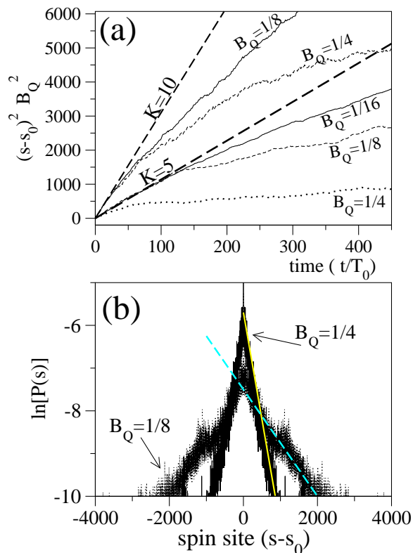
FIG. 2: (a) Shows that, the rate of spreading of a spin excitation initially at an arbitrary site |s_0\rangle in the chain, at short times, is determined solely by the ‘classical stochasticity parameter’ K_s = 2JT_0 B_Q . At longer times, the spreading saturates. The straight line indicates the behaviour expected of the classical chaotic kicked rotor. The smaller the effective value of Planck’s constant, B_Q , the longer the spin spreads linearly at the ‘classical’ rate. Note that in the accelerator mode regime however, the increase would be quadratic in time, not linear. (b) Shows that at sufficiently long times the spin probability distribution saturates into an exponentially localized form. This is the analogue of Anderson Localization in a disordered metal. P(s) \sim \exp\{-2|s - s_0|/L\} so \ln(P(s)) \sim 2/L takes the characteristic ‘triangular form’. The straight lines correspond to L = \frac{K_s^2}{4B_Q^2} for K_s = 10 and agree well with the numerically calculated distributions.
