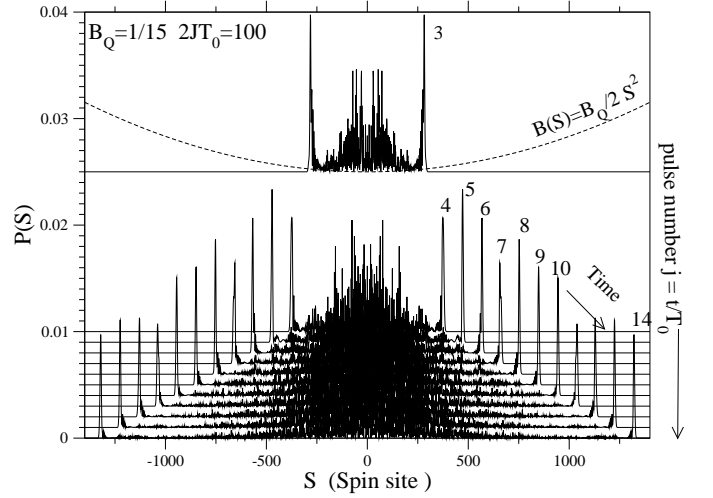
FIG. 1: Time evolution of the state \psi(t=0) = |n_0\rangle (ie initialized with a single spin-excitation at the centre of the chain)-showing the effect of accelerator modes. P(s) represents the probability of finding the excitation at site s . The accelerator modes are the ‘spikes’ at the leading edge of the distribution. They correspond to a counter-propagating pair of coherent states ejected from the centre. We take B_Q = 1/15 and 2JT_0 = 100 . The upper line is at t = 3T_0 ; the lower curves correspond to consecutive periods jT_0 with j = 4, 5, 6, \dots as numbered. The dotted line indicates the form of the parabolic field (scaled by a constant factor) which is pulsed on/off every period at times t = jT_0 . The accelerator modes represent over 25% of the total probability; they advance an equal distance (shown below to be 2\pi/B_Q \simeq 94 spin sites) each period, and after just 3 pulses are well separated from the central, ‘chaotic’ remnant.
