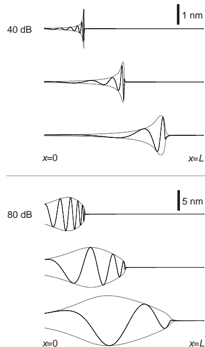
FIG. 1: The active traveling wave on the BM for three different frequencies ( f = 370 Hz, 1.3 kHz & 4.6 kHz) whose corresponding characteristic places are x_r/L = 0.25 (top), 0.5 (center) & 0.75 (bottom). Instantaneous BM displacement h(x, t) (black lines) and wave amplitude H(x) (gray lines) are shown for two stimulus amplitudes, characterized by sound pressure level (SPL). At 40 dB SPL, a sharp resonance occurs at the characteristic place, where the critical oscillators actively drive the response. The resonance is broader at 80 dB SPL, and the peak shifts towards the base of the cochlea. Parameter values: Cochlear dimensions L = 35 mm and l = 1 mm; fluid density \rho = 10^3 kg/m 3 ; parameters governing the frequencies of the active oscillators \omega_0 = 10^5 s -1 and d = 7 mm, providing a frequency range of 100 Hz–16 kHz. We choose \alpha = 10^4 Pa/ms, which implies a volumetric stiffness of the BM varying in the range 6 \times 10^6 - 10^9 Pa/m. There is only one free parameter in our calculations, \beta = 10^{23} Pa/m 3 , which we choose to fit the nonlinearity of the response according to sound pressure level (SPL). For simplicity, it is assumed that the middle ear raises sound pressures by 20 dB, independent of frequency.
