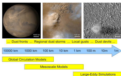
Figure 1: Typical dust lifting events, relevant spatial scales and meteorological models suitable for their analysis.
