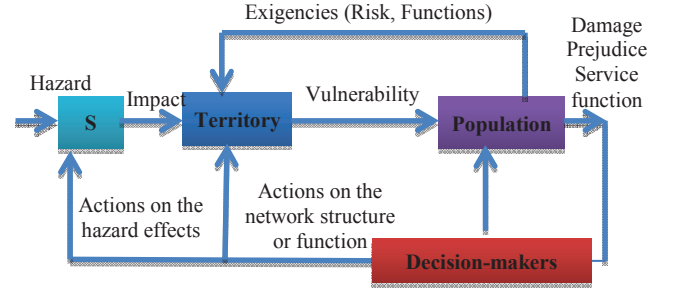
Figure 9 : Vulnerability model
