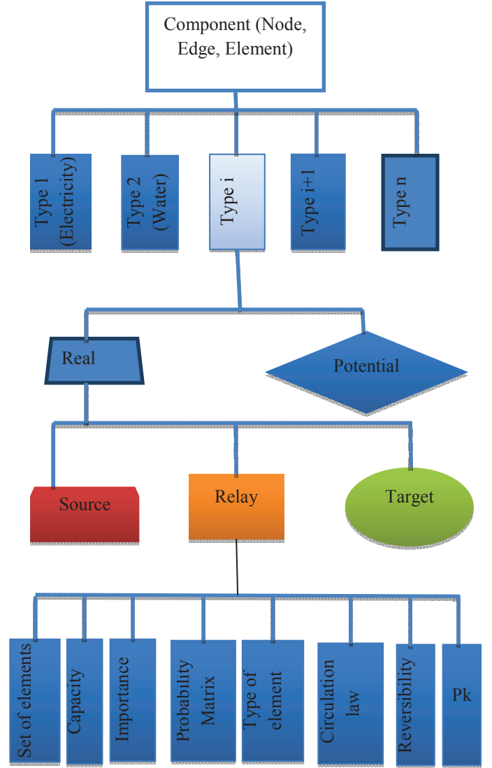
Figure 7: Element class
