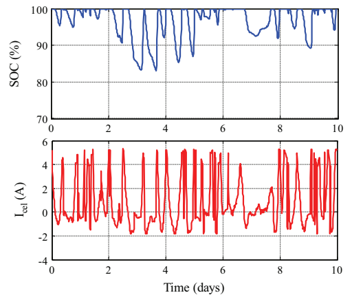
Fig. 11. SOC and I_{\text{cel}} evolutions for the optimal solution.
