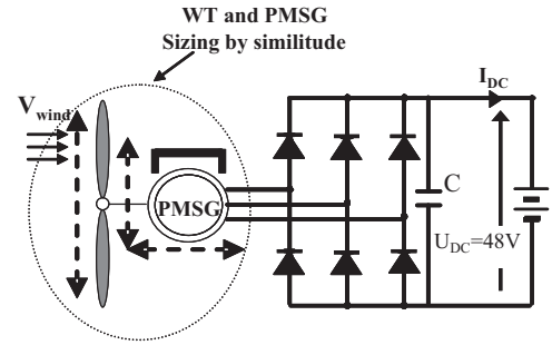
Fig. 5. Passive WT synoptic.
