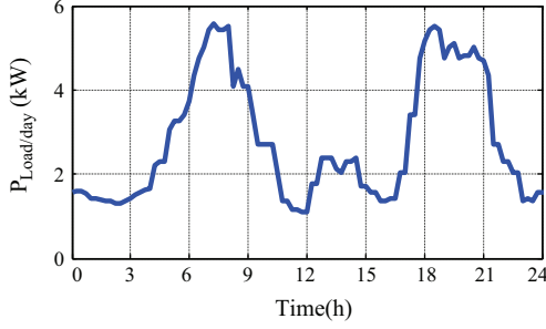
Fig. 2. Typical farm load profile for one day.
