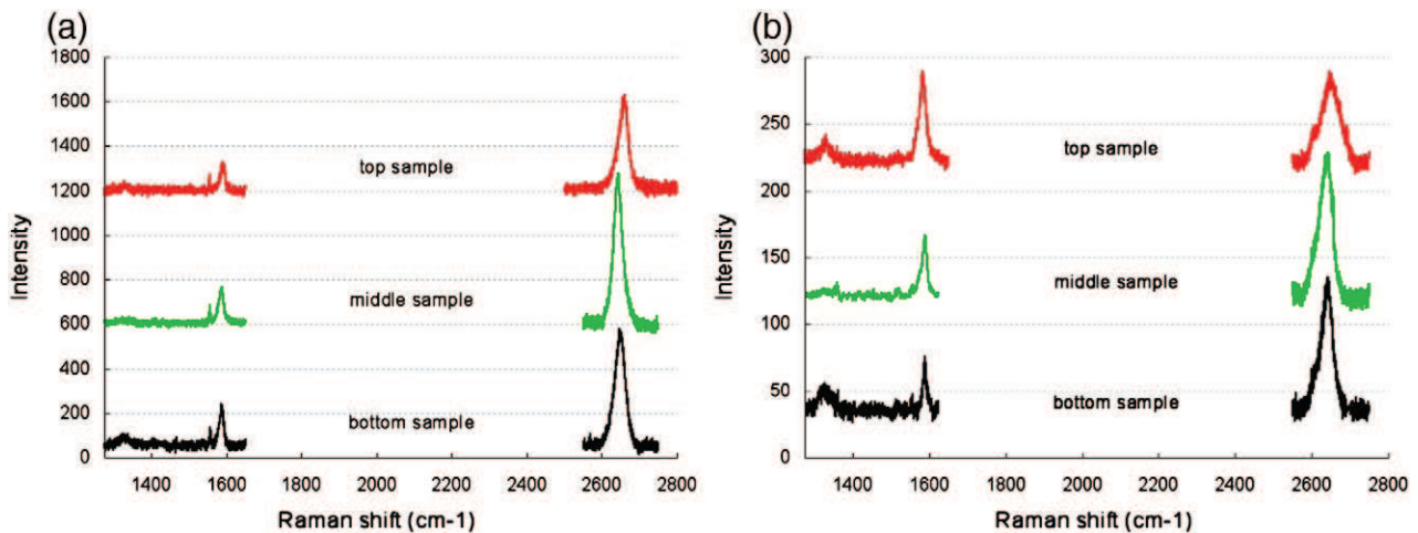
Fig. 4. Raman spectra for hydrogen/methane ratios equal to (a) 800, (b) 400 for 20 ppm of methane.
