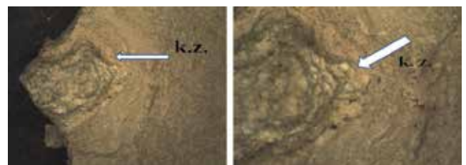
Figure 7. Contact zone *(k.z.) development between the old mortar sample TBM1 and the newly developed mortar DM 3 formed with the pozzolanic material Pozz3
