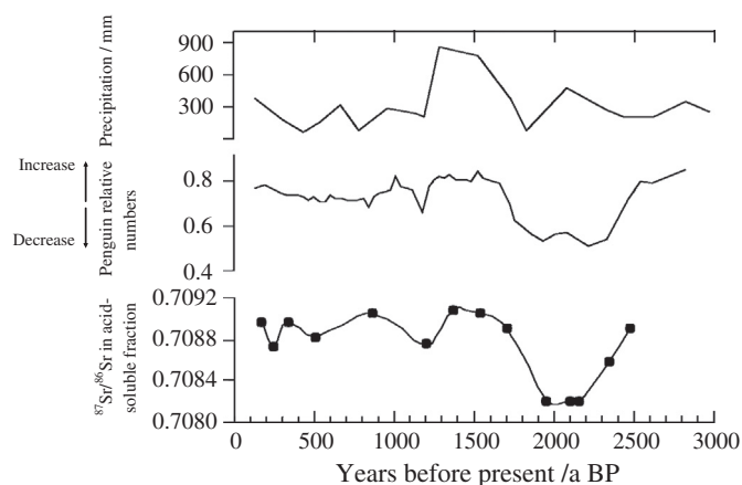
Fig. 2. Changes of ^{87}\text{Sr}/^{86}\text{Sr} ratio in the acid-soluble fraction of Y2 lake sediments (lower curve) (Sun et al., 2005a) and the inferred historical penguin populations (middle curve) on Ardley Island (Sun et al., 2000a) correlated well with local inferred precipitation (upper curve; Zhao, 1991).
