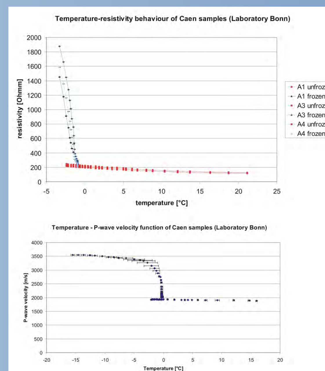
Figure 7: Resistivity and p-wave velocity as functions of temperature for a sample of Tuffeau Chalk derived from calibration measurements.
