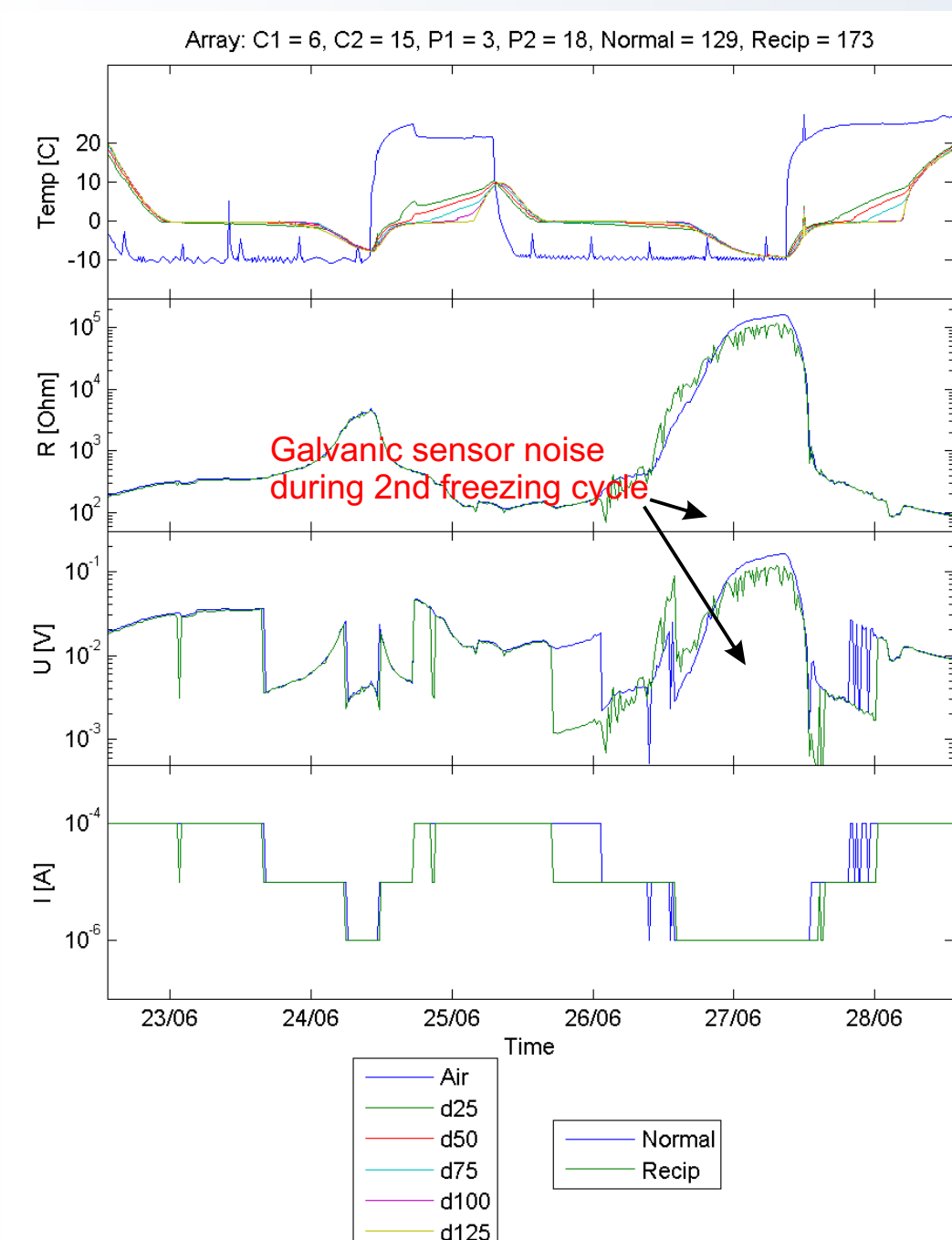
Figure 3: Resistance measurements over time with conventional galvanic electrodes during freeze-thaw experiment on a rock sample
