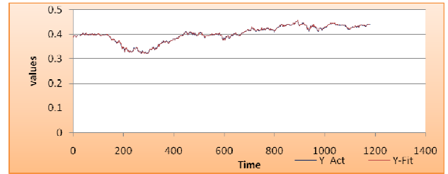
Fig. 14 The plot actual Tala/USD against the fitted value with lag 1
