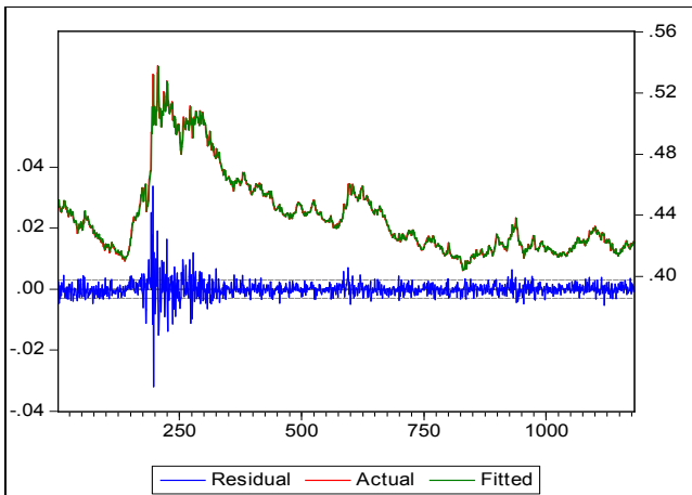
Fig. 4 Residual analysis from the regression of Tala/AUD
