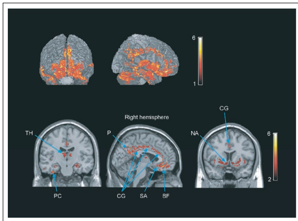
Figure 4. Correlation of hippocampal volume with local gray matter (LGM) amount based on voxel-based morphometry. Top, displays the data overlaid on a “glass brain,” demonstrating the correlation of widespread limbic areas with hippocampal volume. Threshold t = 2.74 (corresponding to p < .005 , uncorrected), cluster size > 150 suprathreshold voxels. Data set smoothed with a Gaussian kernel of 2 mm full width half maximum. BF = basal forebrain; CG = cingulate gyrus; HC = hippocampus; MO = medial orbitofrontal cortex; NA = nucleus accumbens; P = precuneus; PC = perirhinal cortex; SA = subcallosal area; TH = thalamus. All images in radiological convention (left is right).
