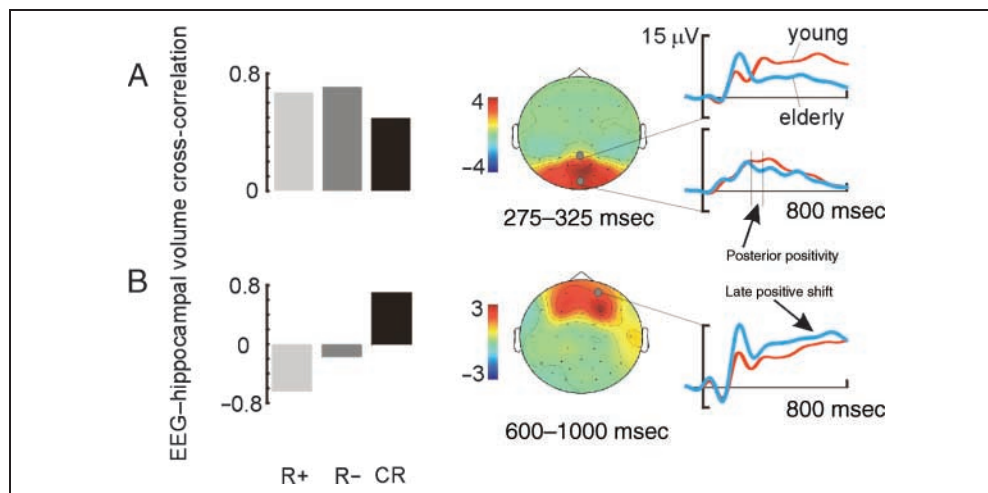
Figure 3. Partial least squares (PLS) analyses of the relation of hippocampal volumes to ERPs in the elderly. (A) PLS with ERP voltages of the elderly elicited by all event classes. Bars on the left depict cross-correlation values of structural data and the topographic map displayed on the right. The topographical map displays the bootstrap ratios (BR, equivalent to z scores; absolute values higher than 1.96 can be considered reliable) for the brain salience of this pattern (latent variable [LV]). The parietal ERPs that are collapsed over all response and stimulus classes and that show the effect revealed in the PLS analysis are displayed on the right. (B) Equivalent to (A), but this time ERPs were normalized before being entered into PLS. The patterns separate CRs from R+ and R-.
