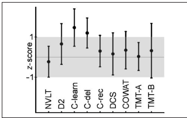
Figure 2. Neuropsychological performance of the elderly subjects. Depicted are group mean and standard deviation for every test after z transformation with respect to the appropriate norms (adjusted for age and education). Tests: Non Verbal Learning Test (NVLT), D2 Test of Attention (D2), California Verbal Learning Test (C-learn, C-del, C-rec), “Diagnosticum für Cerebralschädigung” (DCS), Controlled Oral Word Association Test (COWAT), Trail Making Test Part A and B (TMT-A, TMT-B).
