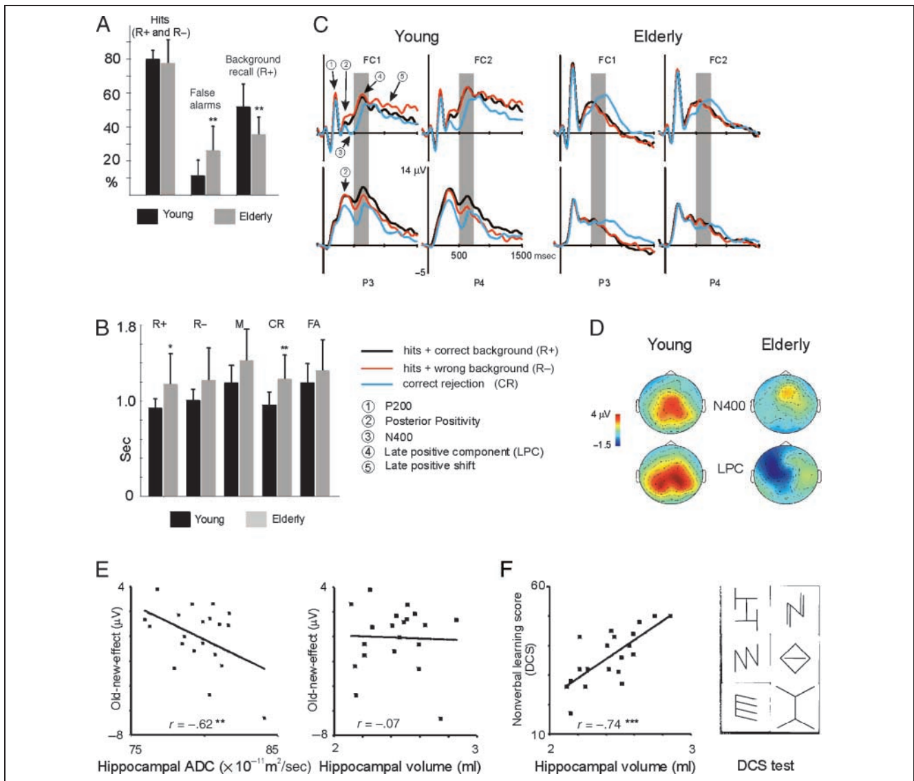
Figure 1. Behavioral and functional results of the ERP paradigm and correlations with hippocampal structure. (A) Correct recognition of studied faces (Hits), “old” responses to new faces (False alarms), correct background recall for hits. (B) Reaction time to all event classes (R+ = correct recognition of a studied face followed by correct background recall; R- = correct recognition of a studied face followed by wrong background recall; M = misses; CR = correct rejections; FA = false alarms). (C) ERPs elicited at frontocentral (FC1 and FC2) and parietal (P3 and P4) electrode sites. The gray bars mark the late positive component (LPC) time window (500–700 msec). (D) Topographical maps of the mean voltage difference between ERPs for hits + correct background recall and correct rejections (correctly identified new faces) in the early (N400, 400–500 msec, top) and the LPC (500–700 msec, bottom) time window for the young (left) and elderly (right). (E) Correlation of hippocampal diffusion (apparent diffusion coefficient [ADC]) and hippocampal volume and the left parietal (P3) ERP difference between hits + correct background recall and correct rejections in the LPC time window. (F) Correlation of nonverbal learning performance (DCS test) with hippocampal volume in the elderly (left) and six example configurations that have to be reproduced in the DCS test (right).
