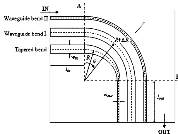
Fig. 1. One basic group of waveguiding components. From smaller to larger radii, each group contained one tapered bend, one waveguide bend with width w_{in} , and one waveguide bend with width w_{out} .
