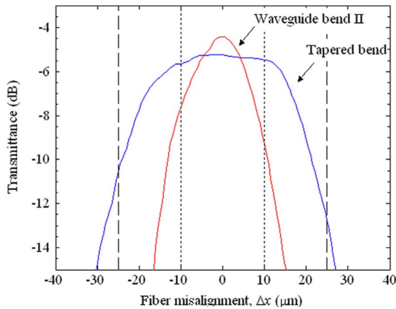
Fig. 3. Coupled power as a function of fiber lateral misalignment from the best coupling position ( \Delta x = 0 ), for a tapered bend and for a waveguide bend II. Dashed lines correspond to the boundaries of the 50- \mu\text{m} -wide entrance of the tapered bend while dotted lines correspond to the boundaries of the 20- \mu\text{m} -wide entrance of the waveguide bend II. Resolution of the scans: 0.5 \mu\text{m} .
