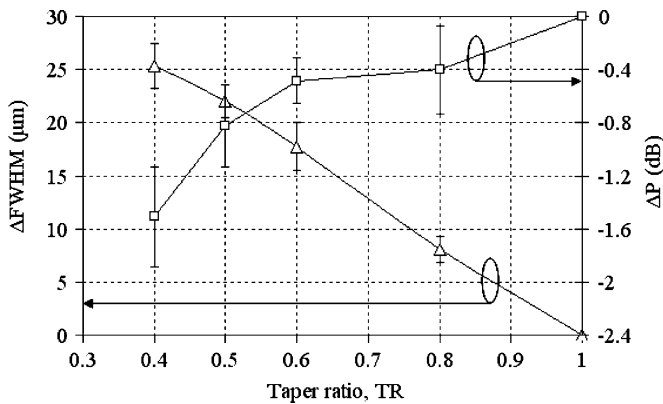
Fig. 4. Mean \Delta FWHM and \Delta P as a function of taper ratio for all tapered bends on the wafer. ( \text{TR} = w_{\text{out}}/w_{\text{in}} .)
