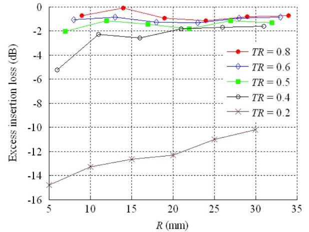
Fig. 2. Excess insertion loss as a function of radius R of curvature for the tapered bends on the wafer for all available TR . ( TR = w_{out}/w_{in} .)
