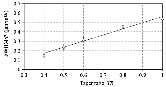
Fig. 5. Maximum coupled power times FWHM misalignment tolerance of tapered waveguide bends as a function of TR. ( \text{TR} = w_{\text{out}}/w_{\text{in}} .)
