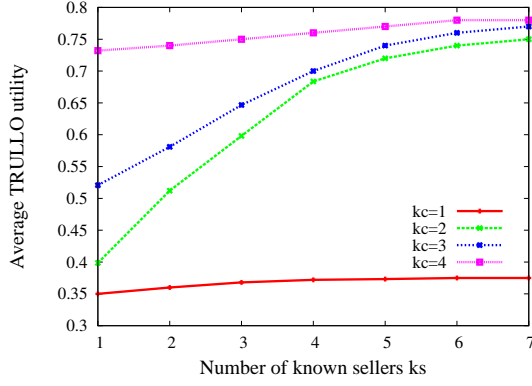
Fig. 6. Average bootstrapping utility for TRULLO versus its input size. Each utility refers to TRULLO bootstrapping trust in a context in which k_s sellers are known in other k_c contexts. We average across all visitors.
