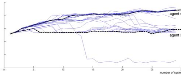
Figure 12. A projection of the agents' ideal means in the world space over time.
