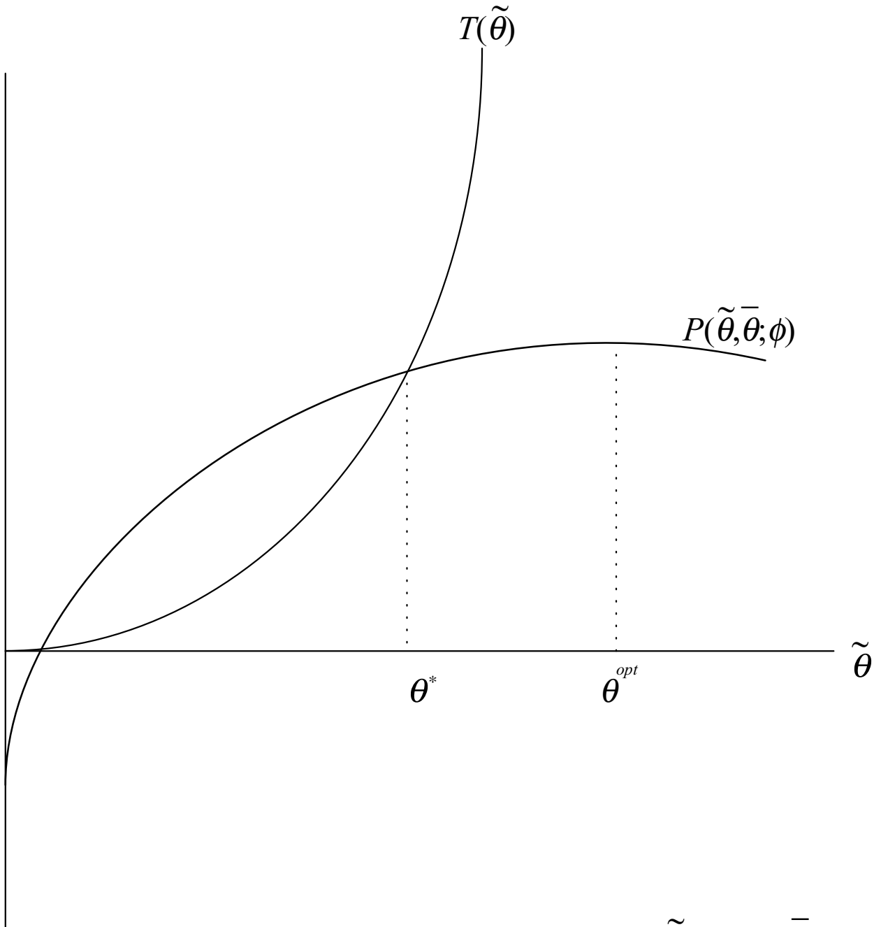
Figure 2: The optimal choice of \tilde{\theta} , given \bar{\theta} .
