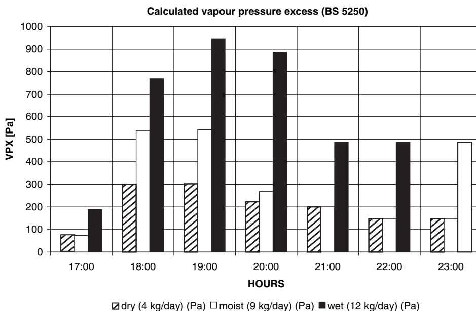
Figure 2 Calculated internal vapour pressure excess (VPX) for dry, moist and wet occupancy
