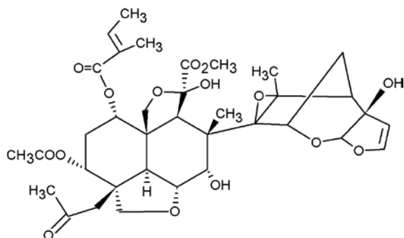
Figure 1 - Azadirachtin molecule.
