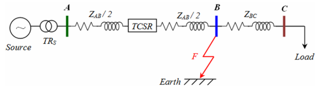
Fig. 3: Transmission line with TCSR.
