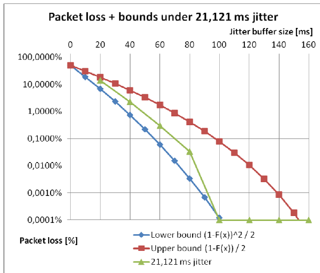
Fig. 4 Measured packet loss vs. calculated upper and lower bounds for 21.121 ms HW jitter and varying buffer size in a lin-log graph showing waterfall-like loss curves up to the expected measurement accuracy
