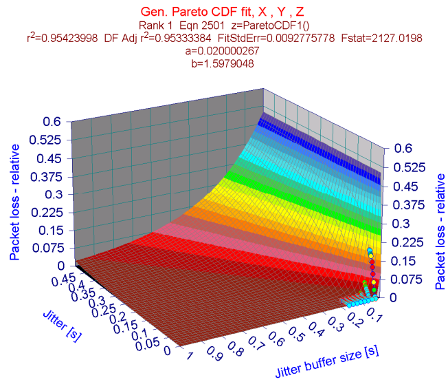
Fig. 10 Larger view on P_{LOSS\_EST} function with \xi > 0
