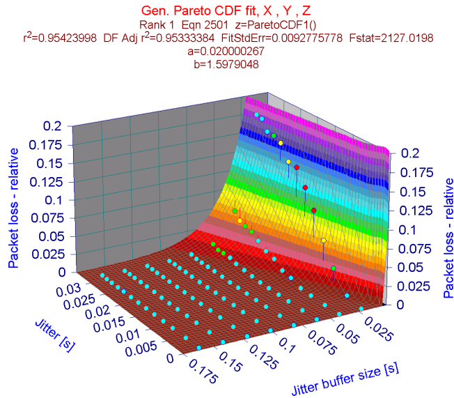
Fig. 9 Larger view on P_{LOSS\_EST} function with \xi > 0
