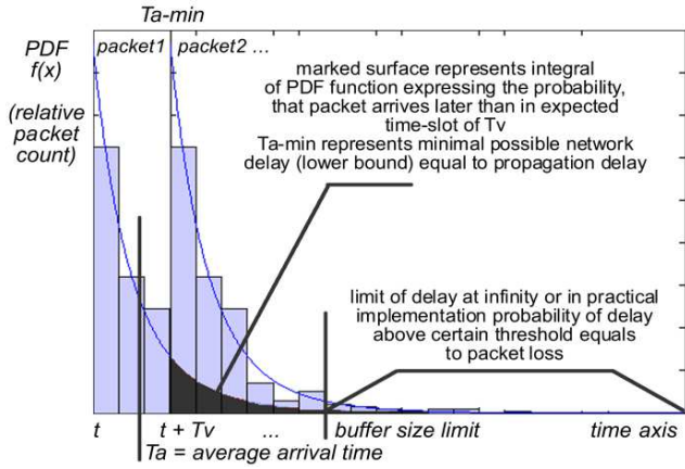
Fig. 2 Distribution of Pareto-related packet arrival times
