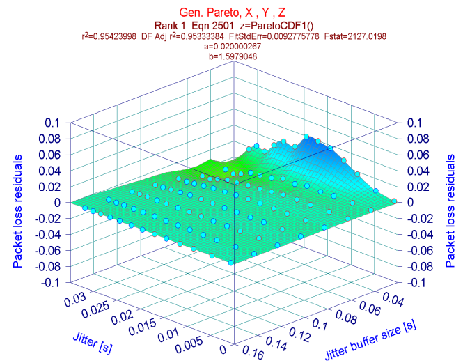
Fig. 11 Absolute residuals of P_{LOSS\_EST} function with \xi > 0
