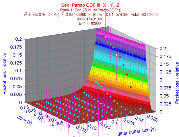
Fig. 6 Optimized P_{LOSS\_EST} function with \xi < 0
