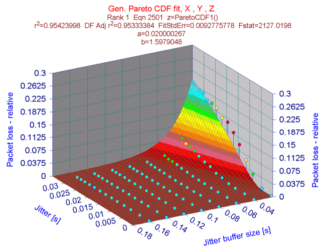
Fig. 8 Optimized P_{LOSS\_EST} function with \xi > 0
