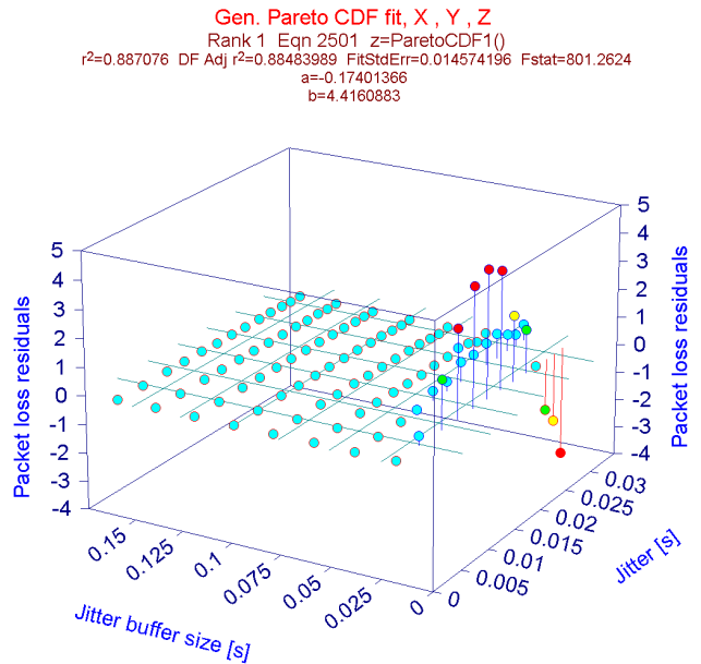
Fig. 5 Residuals of P_{LOSS\_EST} function with \xi < 0
