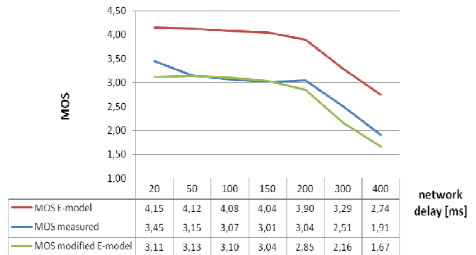
Fig. 1 Comparison of MOS estimates for G.729 codec at 40 ms RFC jitter and 40 ms buffer size, ideal 0 % packet loss under varying network delay
