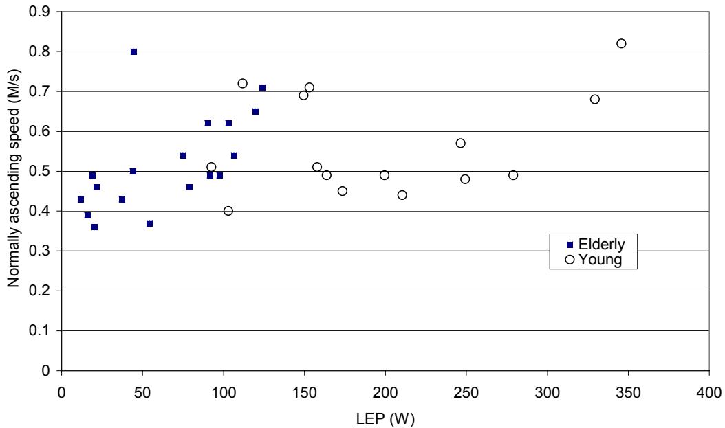
Fig 10. Relation between LEP and normally ascending speed (horizontal speed, Stair 2)
