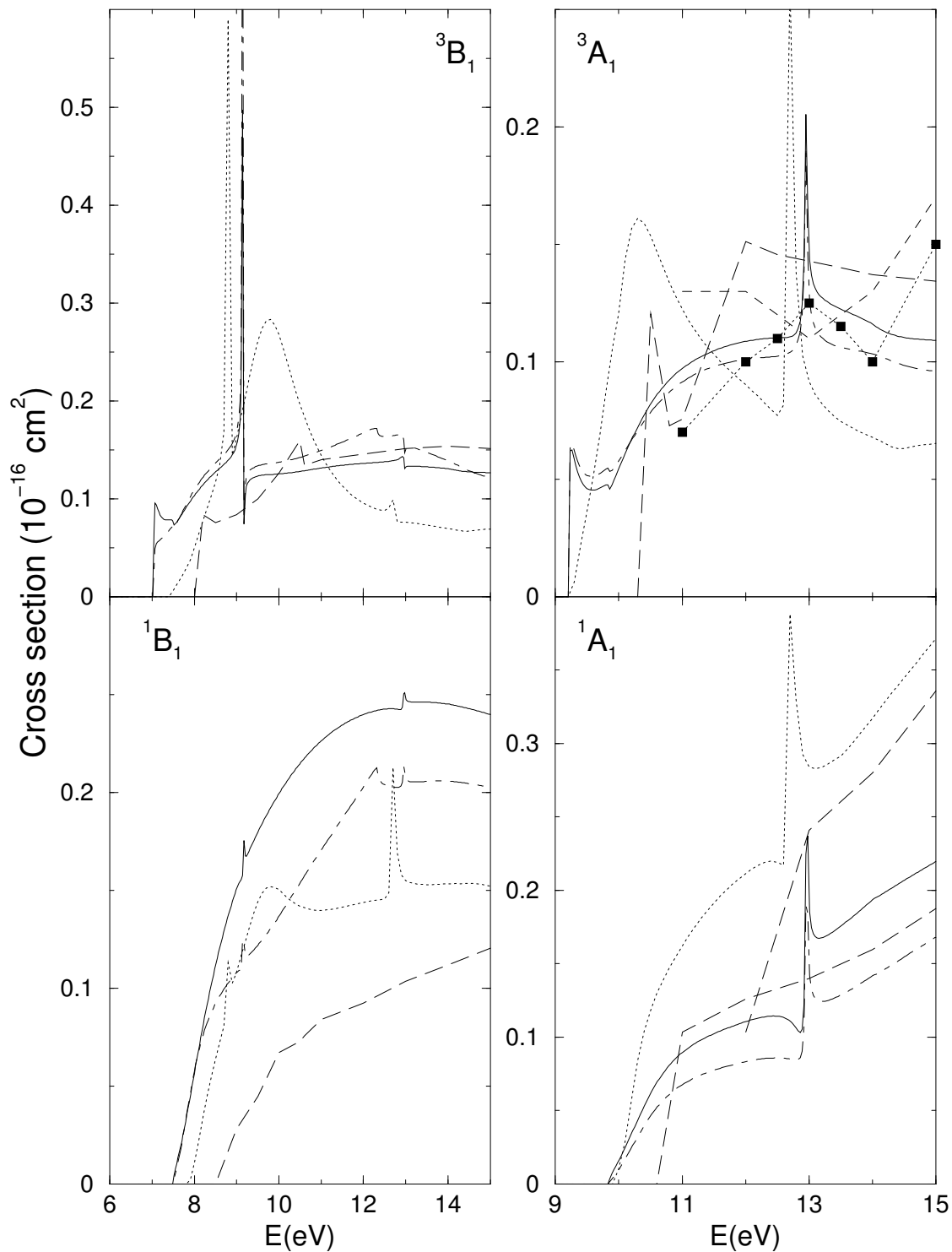
Figure 3. Fixed-nuclei cross sections for excitation into the four lowest excited states of \text{H}_2\text{O} indicated in the figures. Full lines: this work, model (a); dotted-dashed line: this work, model (b); dotted line: Morgan (1998); long-dashed line: Gil et al (1994); dashed-line: Pritchard et al (1990) and dotted-line with squares: Lee et al (1993).
