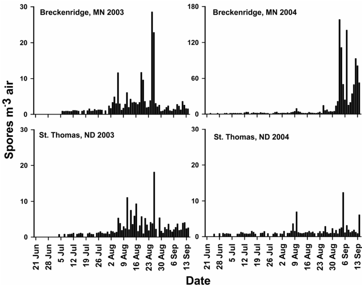
Fig. 1. Daily number of Cercospora beticola spores m^{-3} of air collected with volumetric spore traps in sugar beet fields during 2003 and 2004 at Breckenridge, Minnesota (MN) and at St. Thomas, North Dakota (ND).
