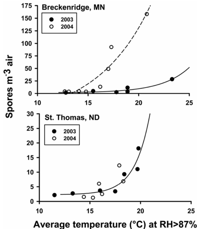
Fig. 2. Relationship between daily mean hourly number of Cercospora beticola spores m -3 of air and average temperature (°C) of daily hours when relative humidity (RH) was greater than 87% in sugar beet fields in 2003 and 2004 at Breckenridge, Minnesota (MN) and at St. Thomas, North Dakota (ND). Each data point represents peak of daily hourly concentration of C. beticola spores per cubic meter of air. The fitted exponential equations at Breckenridge, MN are y = 1.59 + 0.0049 \times 1.447^x with R^2 = 86.5\% and P < 0.05 in 2003, and y = -53.5 + 4.50 \times 1.204^x with R^2 = 87.0\% and P < 0.01 in 2004. The fitted exponential equation at St Thomas, ND is y = 2.28 + 0.000025 \times 1.944^x with R^2 = 81.3\% and P < 0.05 in 2003. In 2004, the relationship between daily mean hourly number of C. beticola spores/m 3 of air and average temperature was not significant ( P > 0.15 ).
