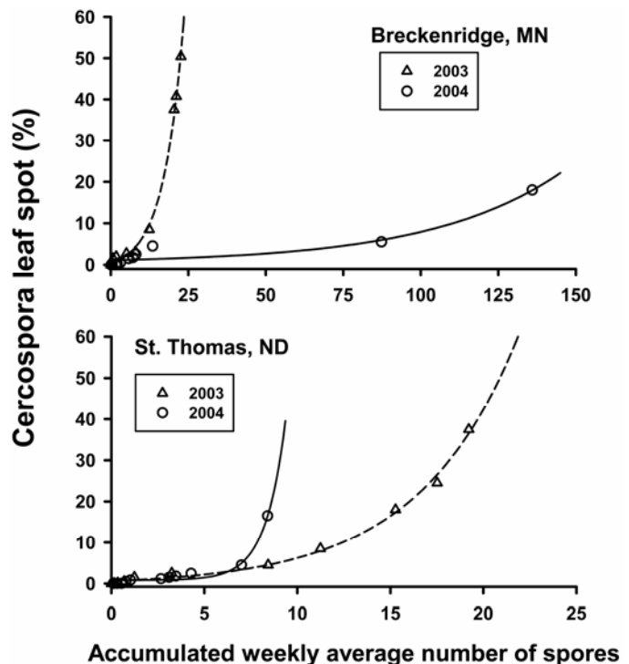
Fig. 3. Relationship between accumulated weekly mean hourly number of Cercospora beticola spores/m 3 of air starting from 5 July and percentage of Cercospora leaf spot severity in sugar beet in 2003 and 2004 at Breckenridge, Minnesota (MN) and at St. Thomas, North Dakota (ND). Each data point is the mean of four observations. The fitted exponential equations at Breckenridge, MN are y = -1.19 + 1.585 \times 1.1671^x with R^2 = 99.7\% and P < 0.001 in 2003, and y = 0.381 + 0.714 \times 1.0283^x with R^2 = 92.4\% and P < 0.001 in 2004. The fitted exponential equations at St Thomas, ND are y = -0.473 + 1.045 \times 1.2039^x with R^2 = 99.3\% and P < 0.001 in 2003, and y = 0.796 + 0.00556 \times 2.574^x with R^2 = 97.2\% and P < 0.001 in 2004.
