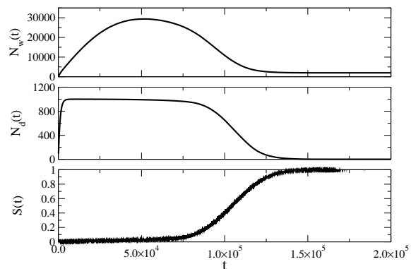
Figure 1: Process evolution - The total number of words in the system, N_w(t) (or total memory used), the number of different words, N_d(t) , and the success rate, S(t) , are plotted as a function of time. The final convergence state is characterized by the presence of the same unique word in the inventories of agents. Thus, at the end of the process, we have N_w(t) = N and N_d(t) = 1 , while the probability of a success is equal to 1 ( S(t) = 1 ). The curves have been obtained averaging over 300 simulation runs for a population of 2 \times 10^3 agents.
